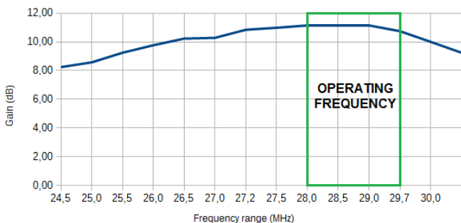
KL200P power Amplifier- Frequency Vs. Gain
