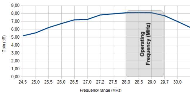
KL35 power Amplifier- Frequency Vs. Gain
